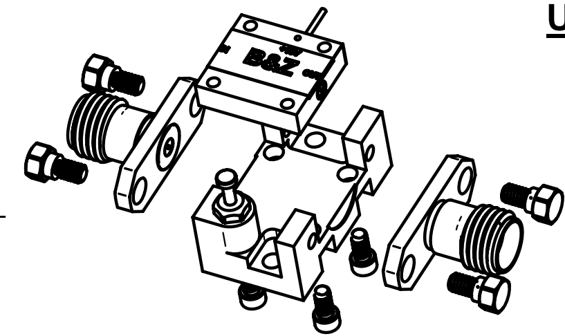
EXPLODED VIEW
